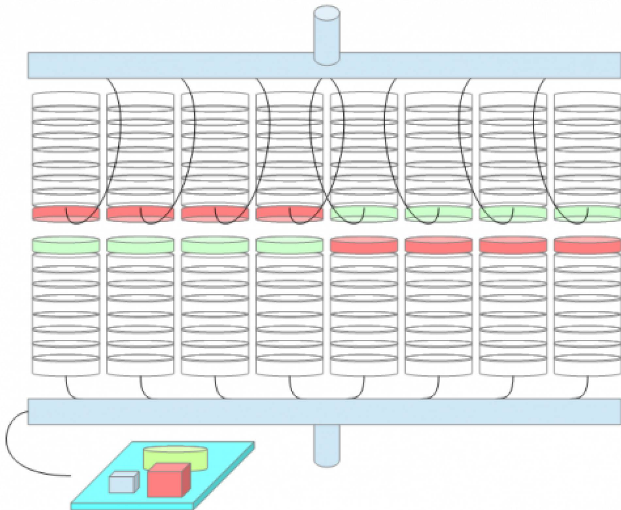
1101 electro magnetic torque converter and acceleration board and software as a clutch operator copyright (c) 2017 Christopher g brown
